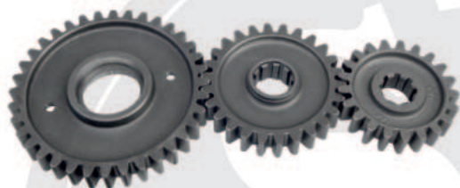
Side Gear Set (36T x 26T x 21T) Part No. NR 1517
