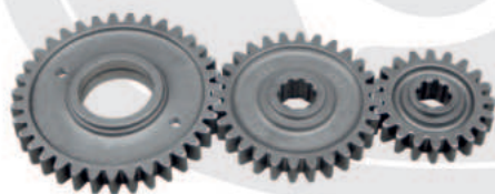
SEMI CHAMPION Side Gear Set 35T x 28T x 20T Big Bore Part No. NR 038
