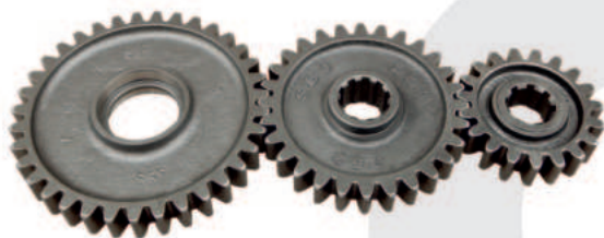
Side Gear 35T x 28T x 19T Part No. NR 1002
