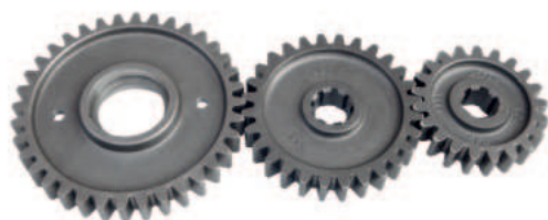
Side Gear Set 21Tx28Tx36T Part No. NR 1745
