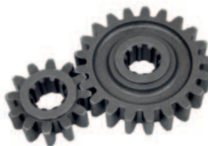
Spur Gear 12x21 Inner 10S Part No. NR 1070
