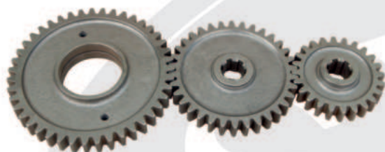
Side Gear 43T x 34T x 24T Part No. NR 2712
