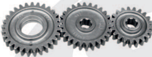
Side Gear Set 21 x 26 x 29 Part No. NR 1841
