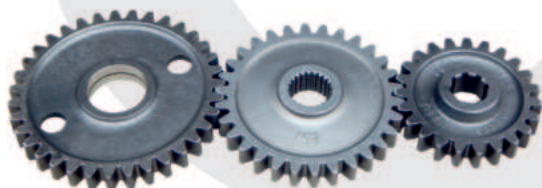
Side Gear Set 35T x 30T x 23T Part No. NR 381
