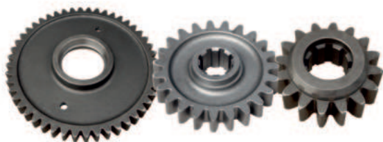
Gear Set 16T x 48T x 23T Part No. NR 1565
