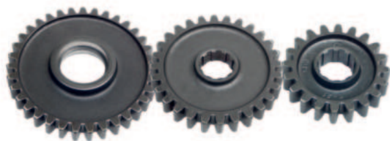
Side Gear Set 35T x 28T x 20T H/D Part No. NR 1545
