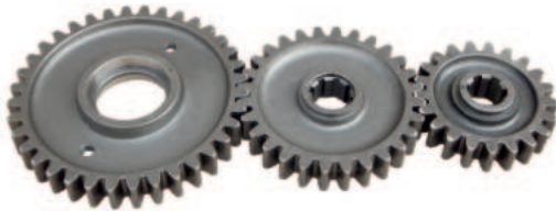
Side Gear Set 36T x 28T x 21T Part No. NR 206
