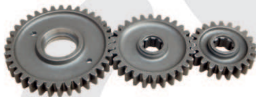
Side Gear Set 36Tx28Tx21T Part No. NR 161
